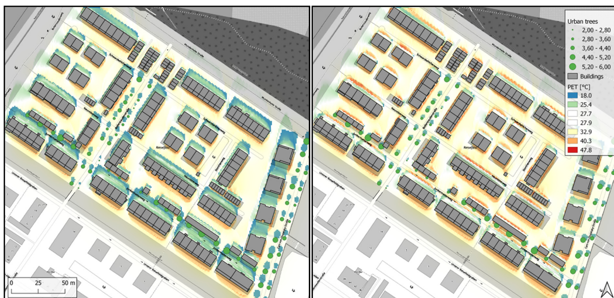
Figure 4. Thermal comfort, based on PET in 1.1 m above ground level for a residential neighborhood in Freiburg, Germany at 13:00 LST, 1st of April (left) and 1st of July (right).
