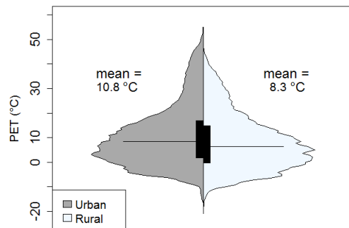
Figure 3. Beanplot for Physiologically Equivalent Temperature ( ^{\circ}\text{C} ). Time period: 1 July 2018 to 28 February 2021 in Freiburg. The distance between the rural and urban station in Freiburg is about four kilometers.
