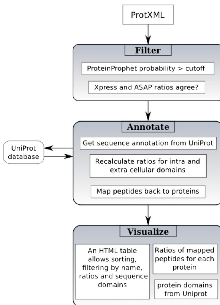
Figure 1 Flowchart depicting the working procedure of the ImproViser tool. The tool accepts a protXML file as input. Using information retrieved from this file, it refers to the UniProt database to obtain selected information and delivers it back to the ImproViser script, which generates a graphical table with all relevant information. This output is then compressed and can be downloaded as a zip file by the user.
